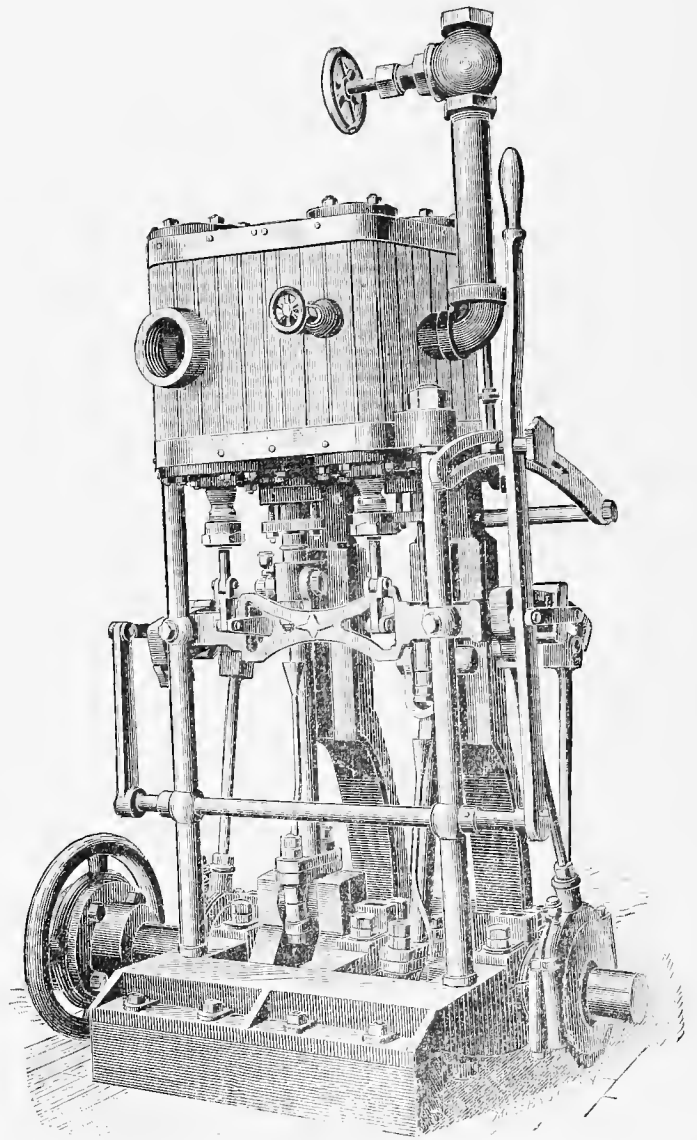
TROMBLEY'S COMPOUND YACHT ENGINE.
